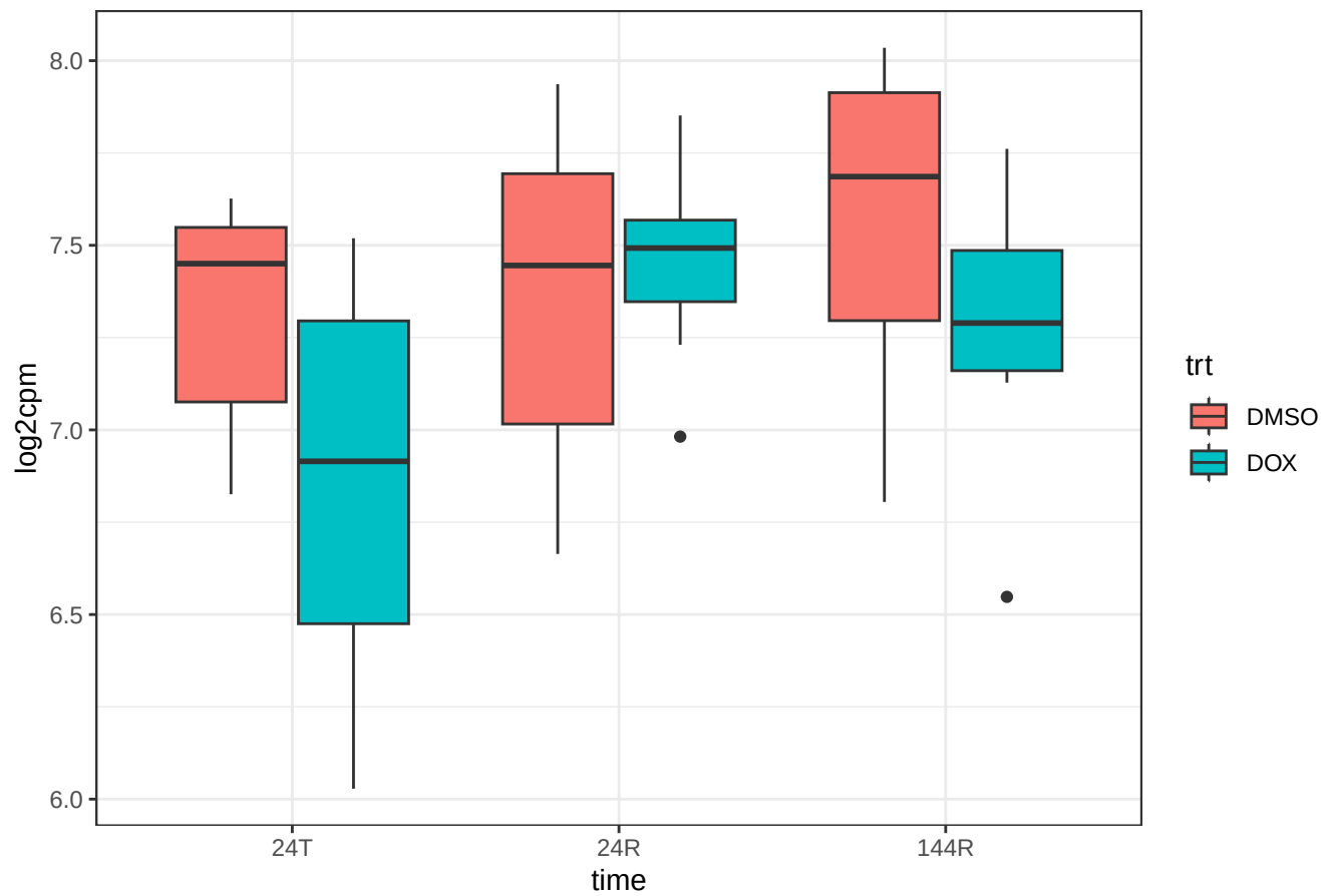
gene 394 ARHGAP5 dist 54817
